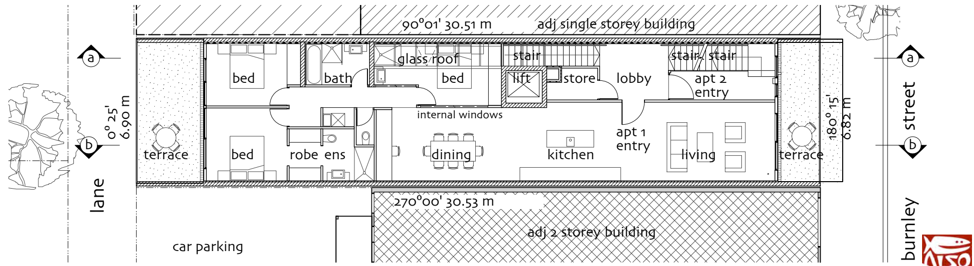
1ST FLOOR PLAN
